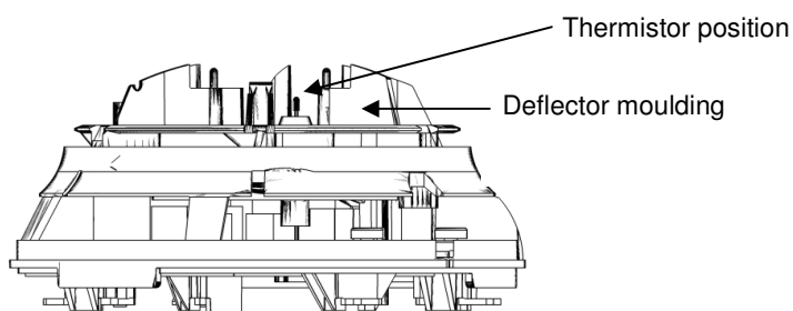
Diagram 3 Re Assembly showing correct thermistor position
